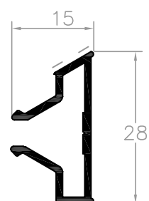
L50817 clip pingadeira
