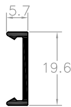
L50807 clip pingadeira
