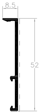
L52767 perfil remate 52 x 8.5
