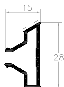
L50817 clip pingadeira
