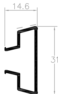
L50811 clip pingadeira
